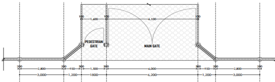
GROUND FLOOR LAYOUT PLAN
