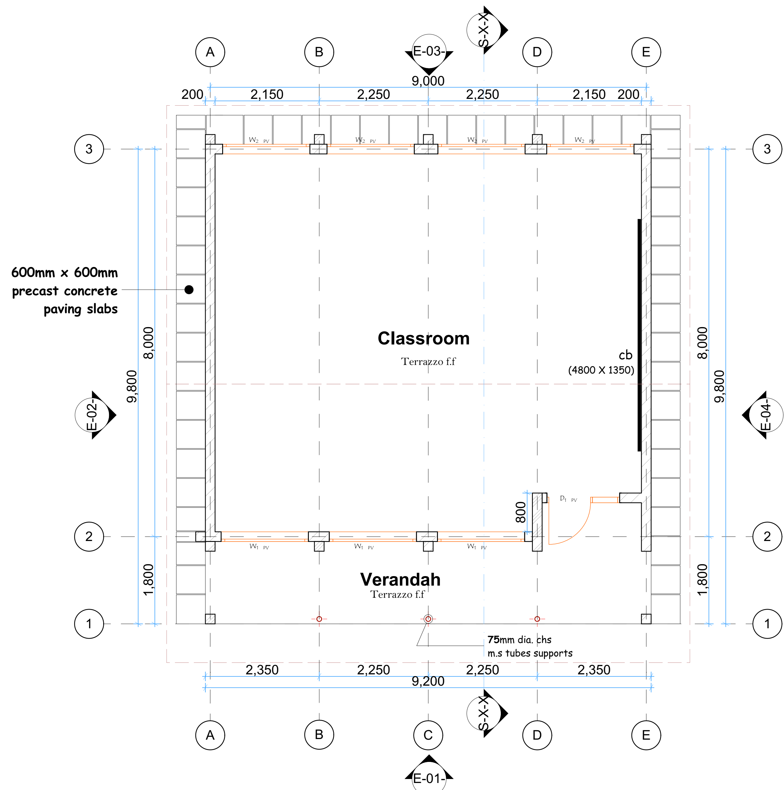
GROUND LAYOUT PLAN SCALE 1:100
