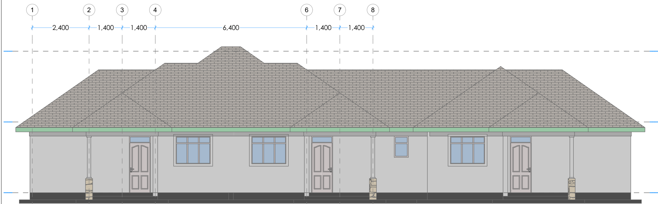
REAR ELEVATION 03
