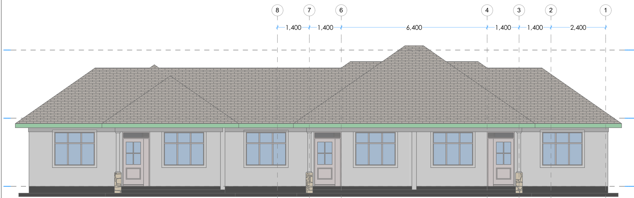
FRONT ELEVATION 01
