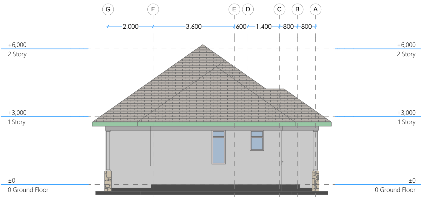
SIDE ELEVATION 02
