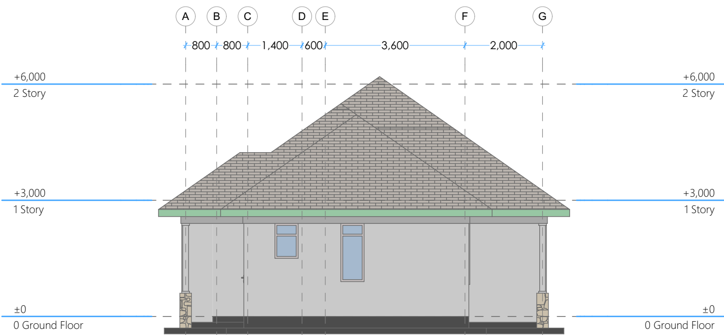
SIDE ELEVATION 04
