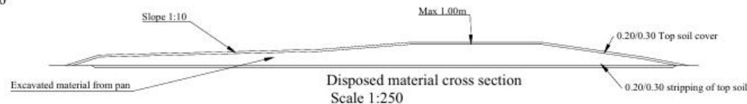
Cross section A-A
