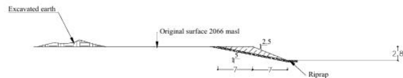
Cross section B-B
