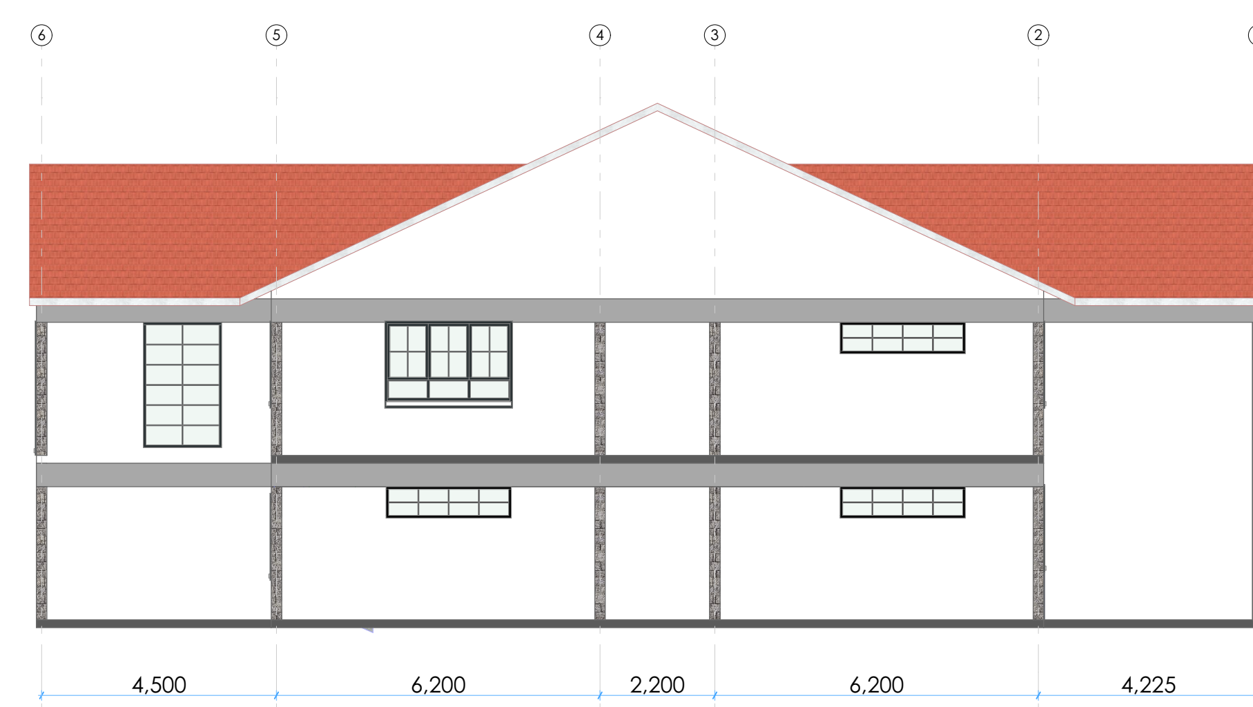
ELEVATION E-2
