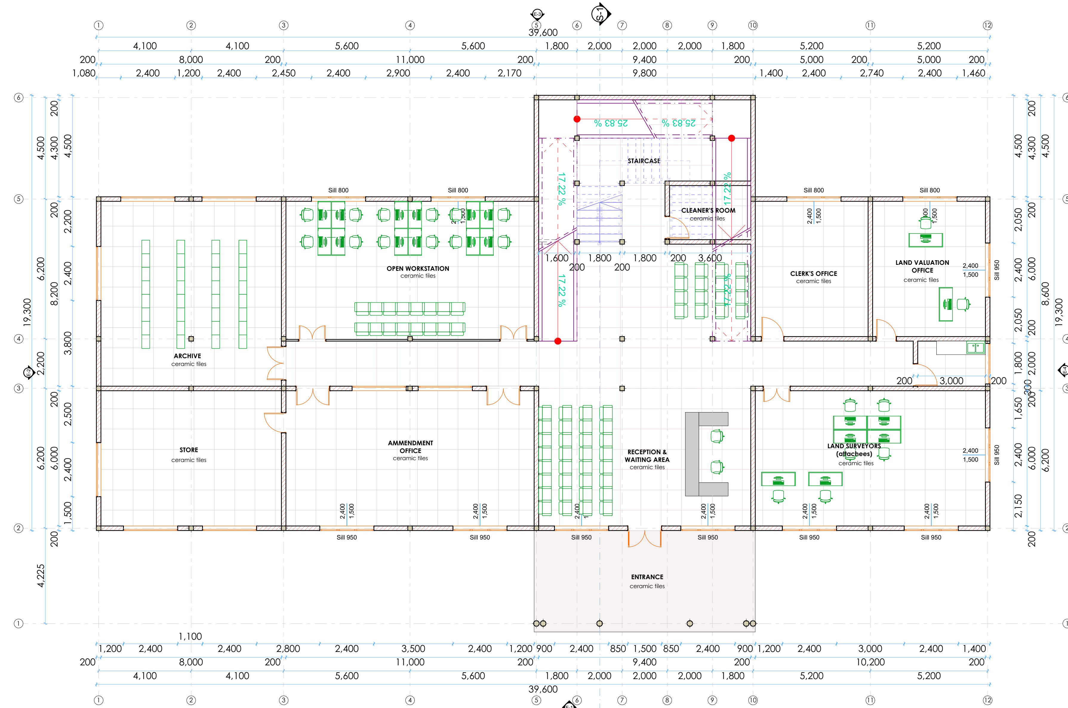
GROUND FLOOR 674 m 2
