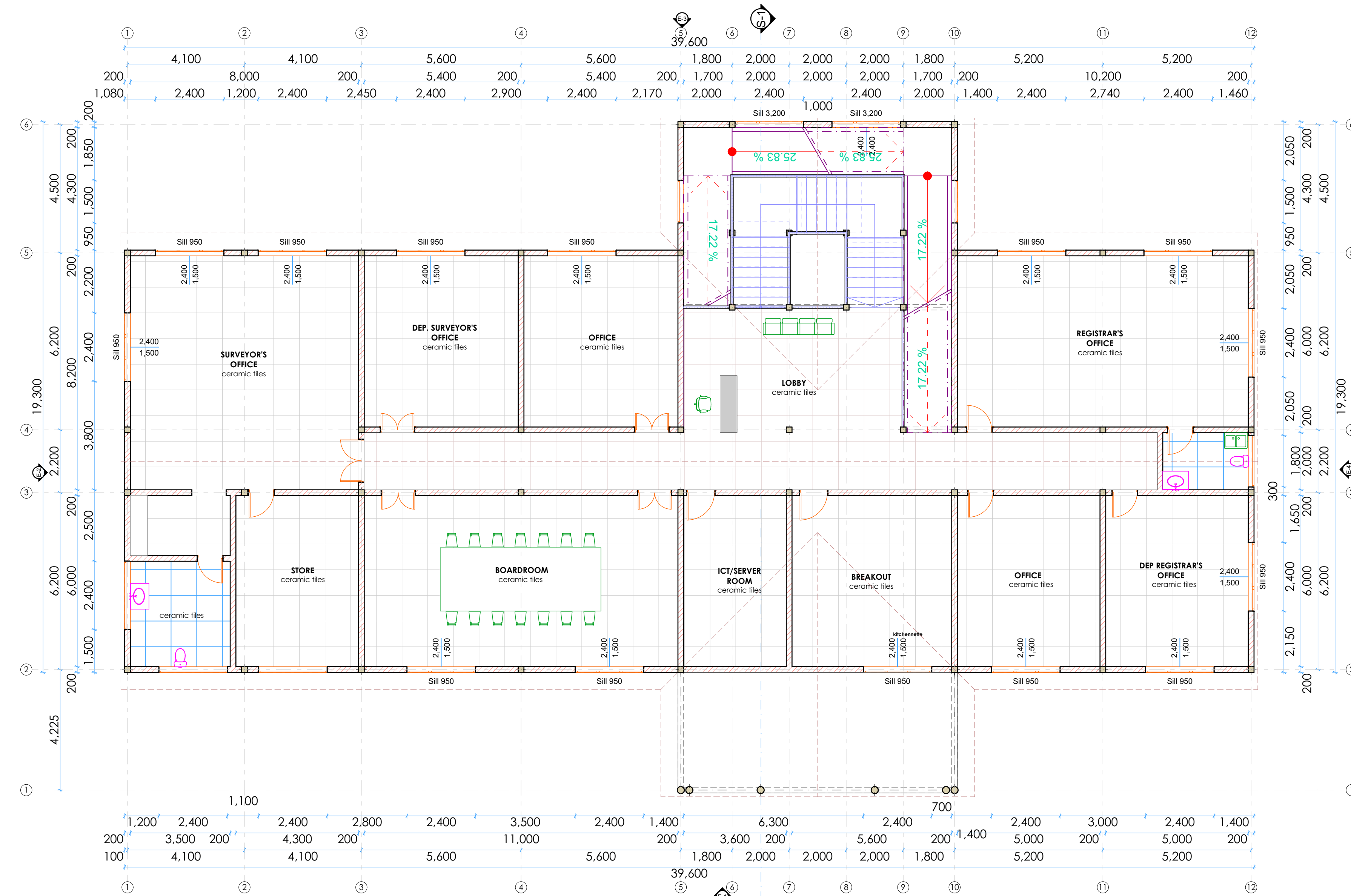
FIRST FLOOR 560 m 2
