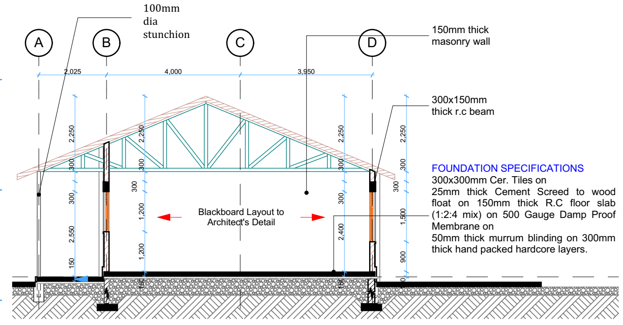
SECTION AA 1:100
