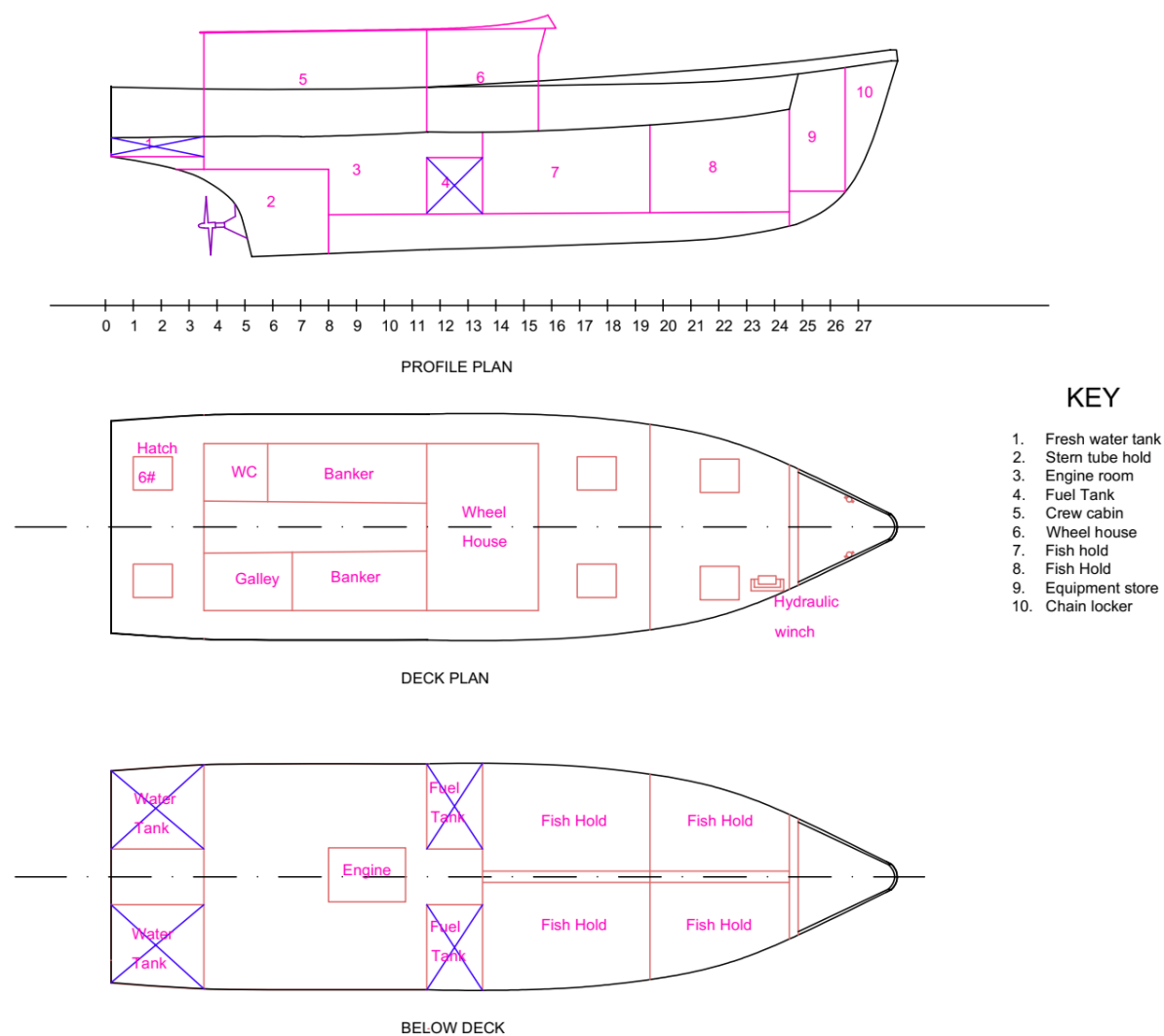
Typical Proposed Fishing Boat for KEMFSED Project
