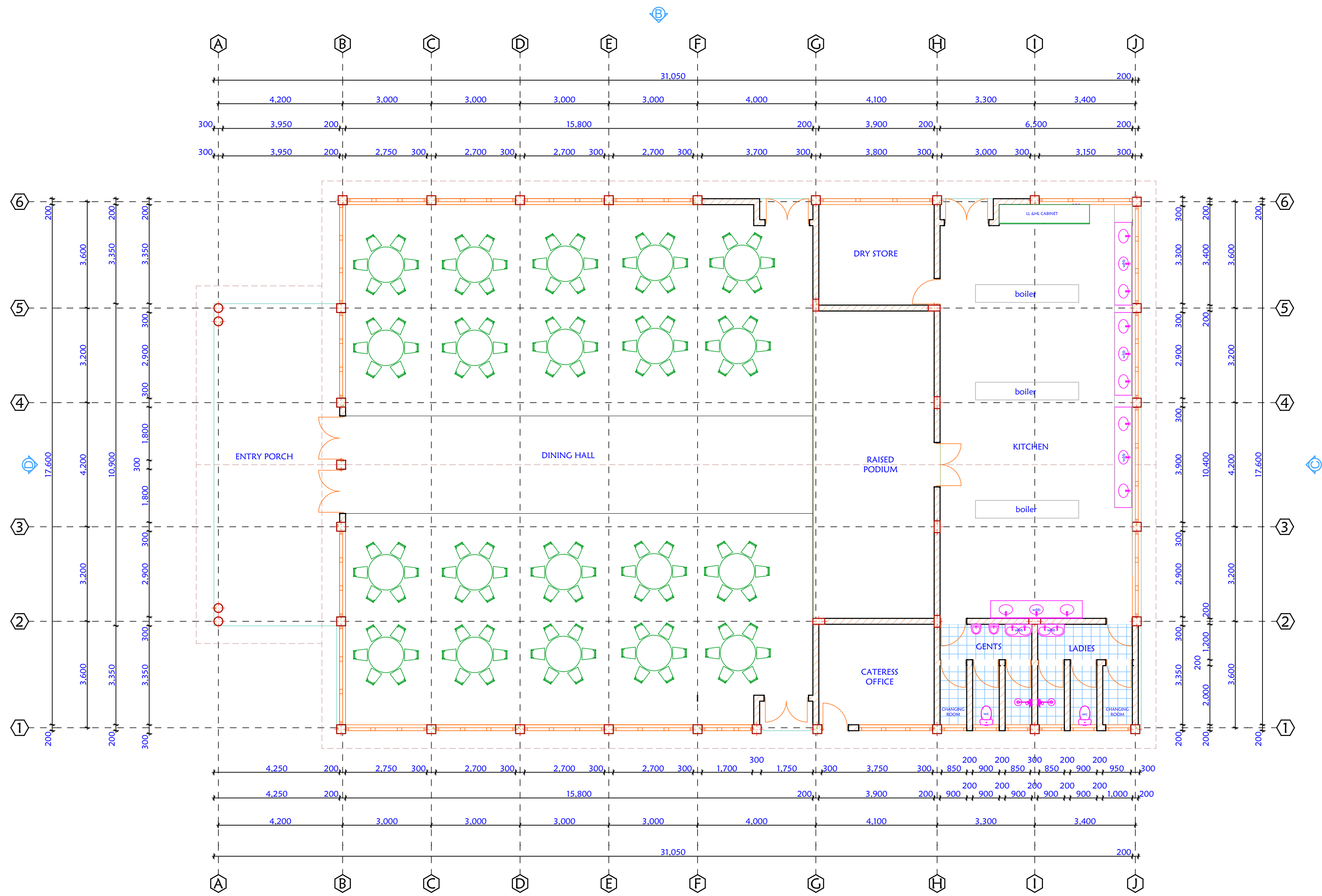
FLOOR PLAN LAYOUT
