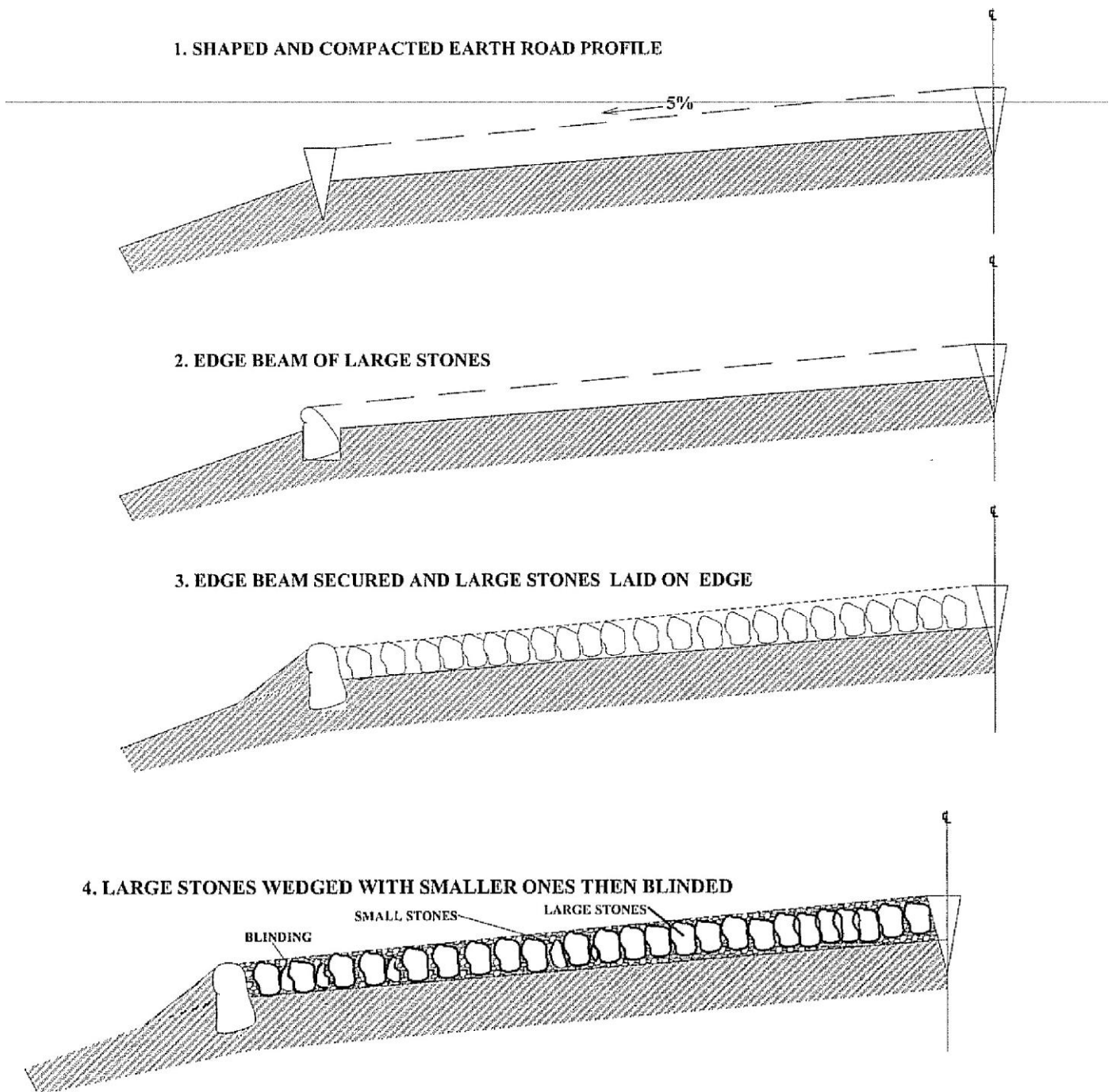
FIGURE C21-HAND PACKED STONE PAVEMENT
